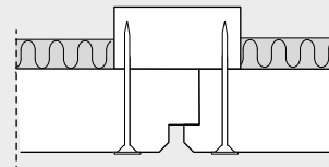
K5-FU Troldtekt Plus With 5 mm bevel and rebate for U-profile
