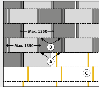
FIG. 3 STRETCHER BOND
